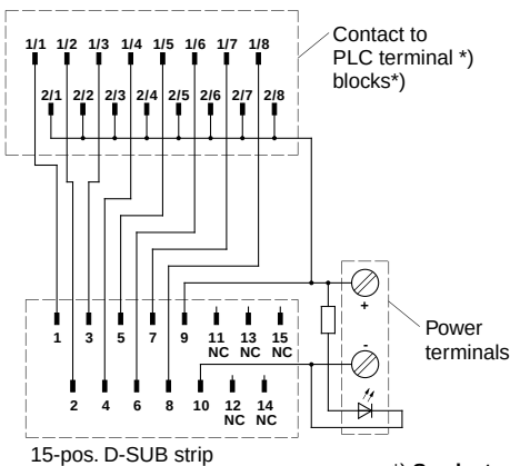
Connection diagram for the PLC-V8/D15S/IN PLC-V8/D15B/IN
