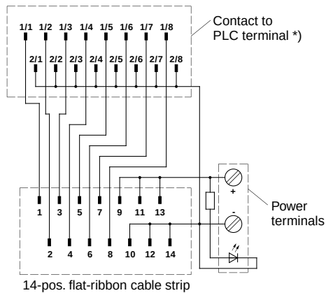
Connection diagram for the PLC-V8/FLK14/OUT
