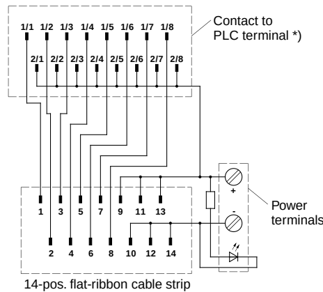
Connection diagram for the PLC-V8/FLK14/IN
