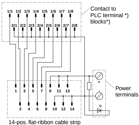
Connection diagram for the PLC-V8L/FLK14/OUT
