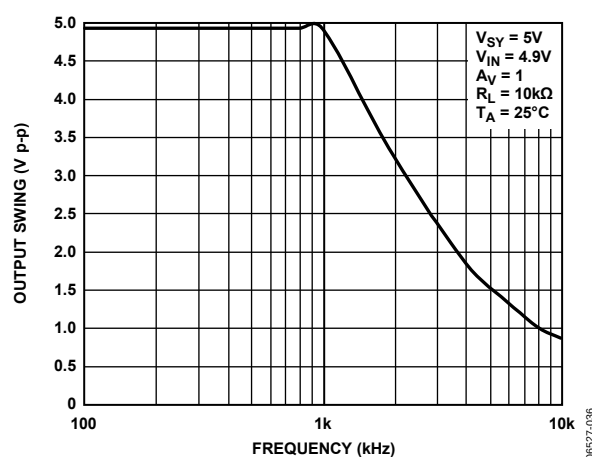
Figure 39. Maximum Output Swing vs. Frequency
