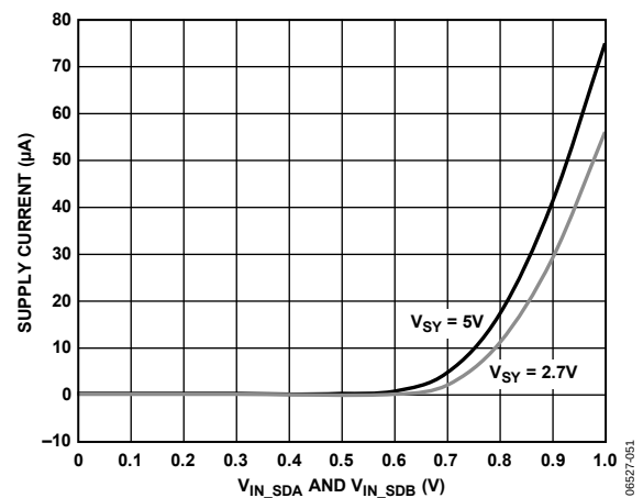
Figure 50. Supply Current Shutdown Mode, AD8647
