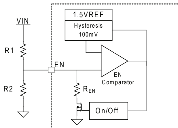
Figure 7 — Enable Input Circuit
