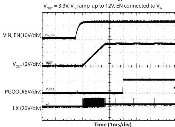
Startup - V IN ramp
