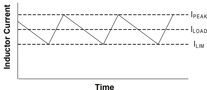
Figure 6 — Valley Current Limit
