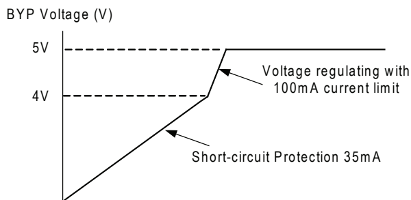
Figure 9 — LDO Start-Up
