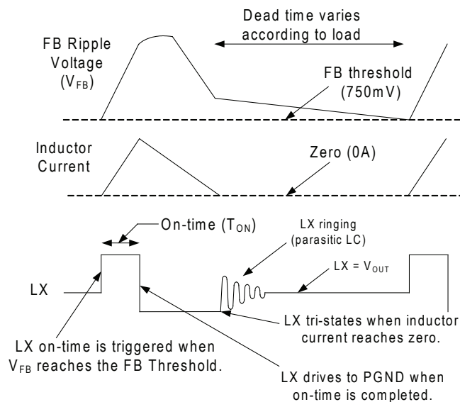
Figure 4 — Power-save Operation
