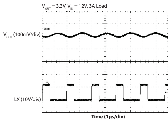
Continuous Mode Switching - 3A Load
