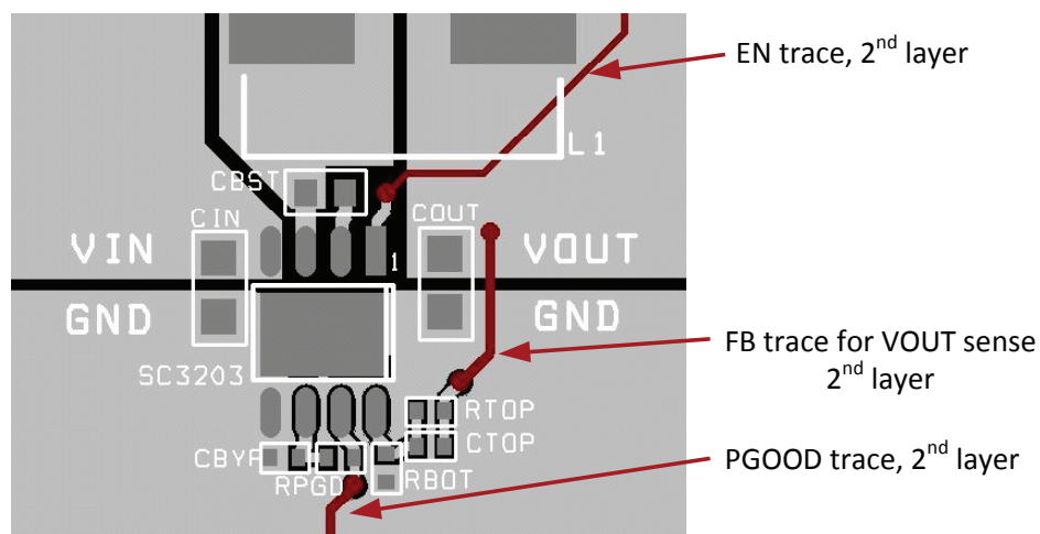
Figure 12 — PCB Layout
