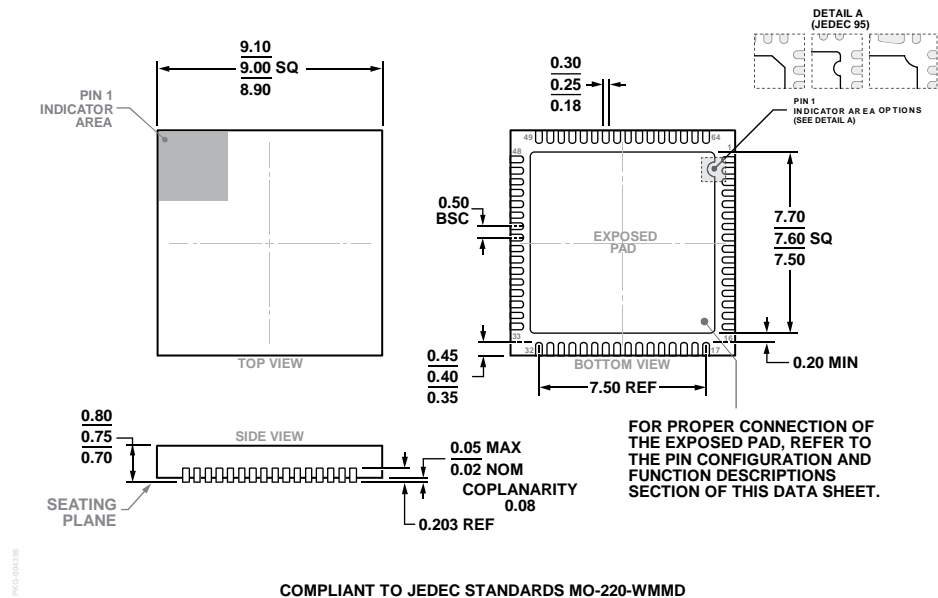
COMPLIANT TO JEDEC STANDARDS MO-220-WMMD Figure 187. 64-Lead Lead Frame Chip Scale Package [LFCSP] 9 mm x 9 mm Body and 0.75 mm Package Height (CP-64-15) Dimensions shown in millimeters
