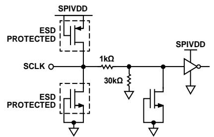
Figure 109. SCLK Input
