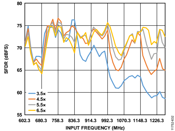
Figure 119. Buffer Current Sweeps, AD9680-1250 (SFDR vs. I_{BUFF} ); 600 \text{ MHz} < f_{IN} < 1300 MHz; Front-End Network Shown in Figure 115
