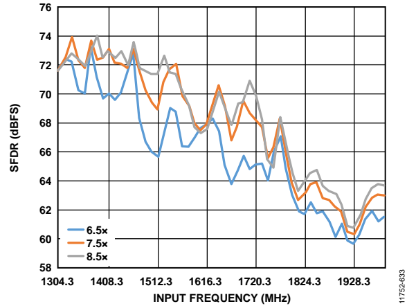
Figure 120. Buffer Current Sweeps, AD9680-1250 (SFDR vs. I_{BUFF} ); 1300 \text{ MHz} < f_{IN} < 2000 MHz; Front-End Network Shown in Figure 115
