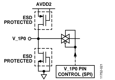
Figure 114. V_1P0 Input/Output
