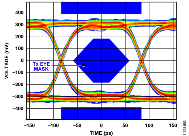
Figure 164. Digital Outputs Data Eye, External 100 Ω Terminations at 6 Gbps
