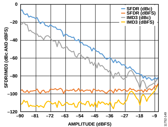
Figure 96. Two-Tone IMD3/SFDR vs. Input Amplitude ( A_{IN} ) with f_{IN1} = 338\text{ MHz} and f_{IN2} = 341\text{ MHz}
