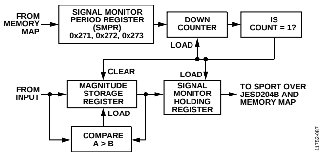
Figure 142. Signal Monitor Block
