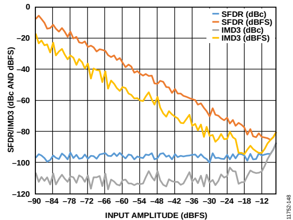
Figure 95. Two-Tone SFDR/IMD3 vs. Input Amplitude ( A_{IN} ) with f_{IN1} = 184\text{ MHz} and f_{IN2} = 187\text{ MHz}
