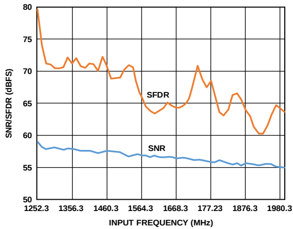
Figure 18. SNR/SFDR vs. f_{IN} ; 1.3 \text{ GHz} < f_{IN} < 2 \text{ GHz} ; Buffer Control 1 (0x018) = 8.5×
