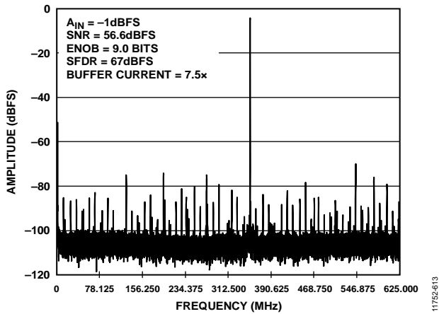
Figure 13. Single-Tone FFT with f_{IN} = 1602.3 \text{ MHz}
