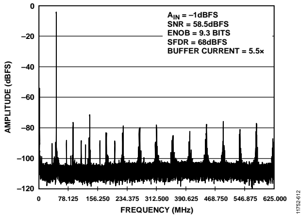
Figure 12. Single-Tone FFT with f_{IN} = 1205.3 \text{ MHz}
