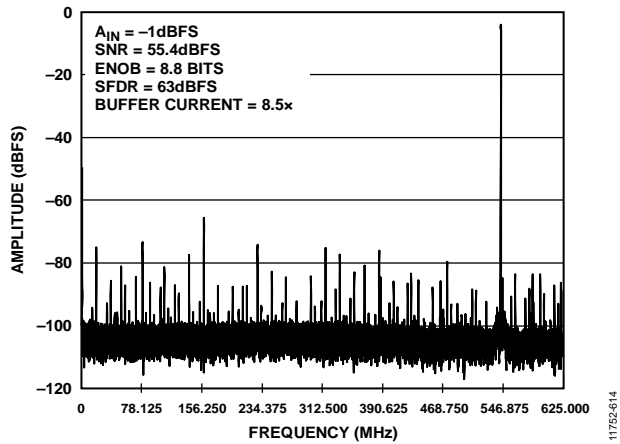
Figure 14. Single-Tone FFT with f_{IN} = 1954.3 \text{ MHz}
