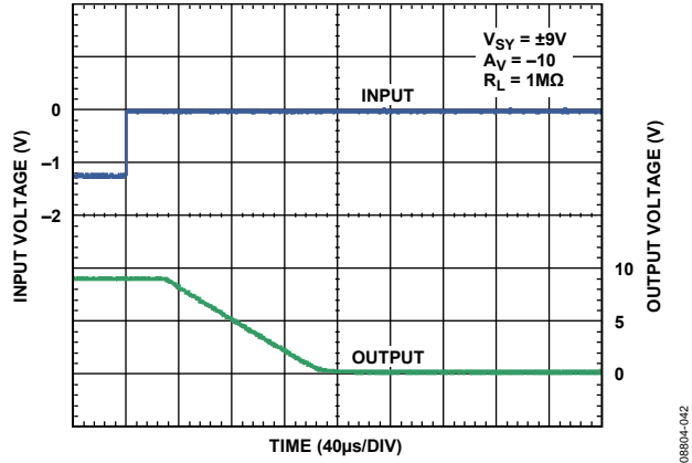
Figure 53. Positive Overload Recovery
