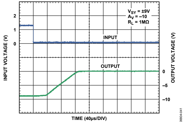
Figure 54. Negative Overload Recovery
