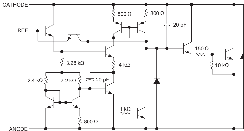
Figure 3. EQUIVALENT SCHEMATIC
