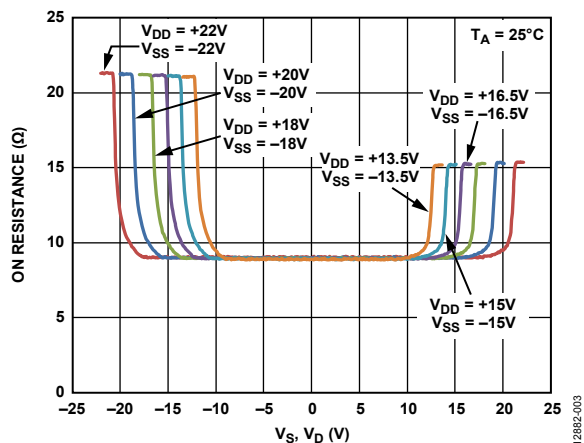
Figure 4. R_{ON} as a Function of V_S and V_D Various Dual Supplies
