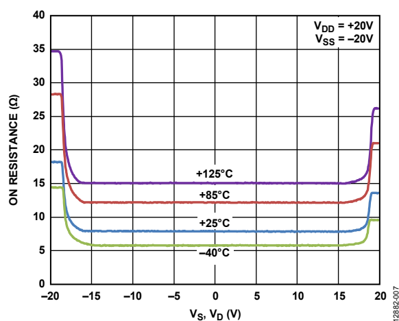
Figure 8. R_{ON} as a Function of V_S and V_D for Different Temperatures, \pm 20\text{V} Dual Supply
