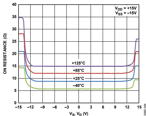
Figure 7. R_{ON} as a Function of V_S and V_D for Different Temperatures, \pm 15\text{V} Dual Supply
