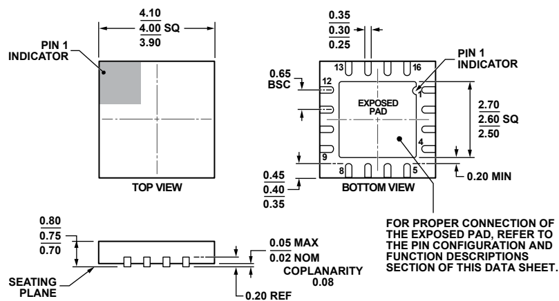
Figure 53. 16-Lead Lead Frame Chip Scale Package [LFCSP_WQ] 4 mm × 4 mm Body, Very Very Thin Quad (CP-16-17)
