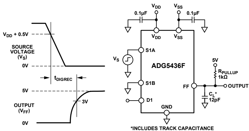
Figure 43. Interrupt Flag Recovery Time, t_{DIGREC} with a 1 k \Omega Pull-Up Resistor
