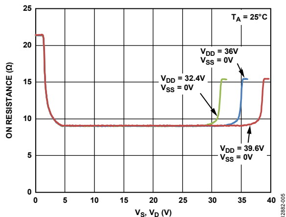
Figure 6. R_{ON} as a Function of V_S and V_D 36 V Single Supply
