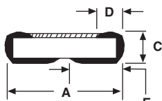
WIDE BOTTOM TERMINAL (W)
