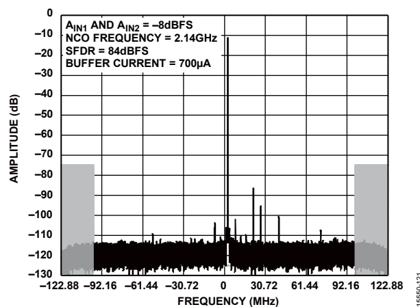
Figure 51. Two-Tone FFT; f_{IN1} = 1846.5 MHz, f_{IN2} = 2142.5 MHz f_{CLK} = 2.4576 GHz; Decimation Ratio = 10, NCO Frequency = 2140 MHz
