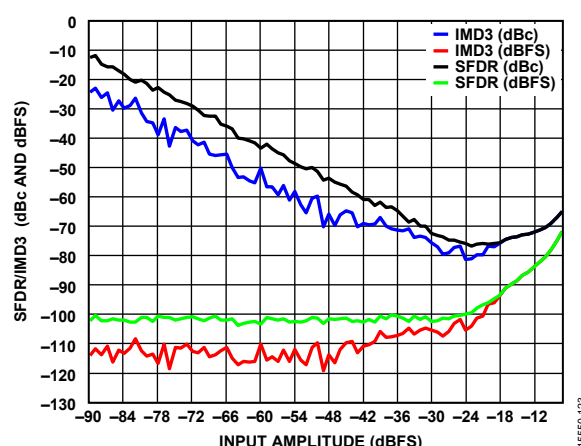
Figure 53. Two-Tone SFDR/IMD3 vs. Input Amplitude ( A_{IN} ) with f_{IN1} = 2137.5 MHz, f_{IN2} = 2142.5 MHz
