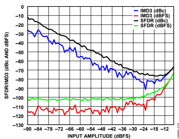
Figure 52. Two-Tone SFDR/IMD3 vs. Input Amplitude ( A_{IN} ) with f_{IN1} = 1841.5 MHz, f_{IN2} = 1846.5 MHz
