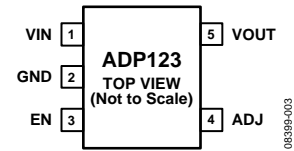
Figure 7. ADP123 TSOT Adjustable Output Pin Configuration
