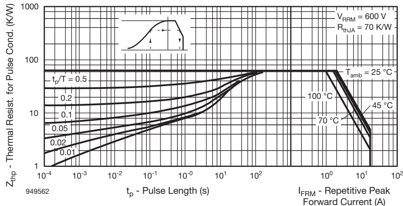
Fig. 7 - Thermal Response
