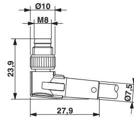
Plug M8 x 1, angled, shielded
