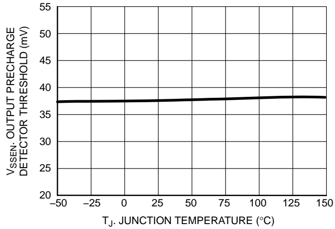
Figure 24. Output Precharge Detector Threshold vs. Junction Temperature
