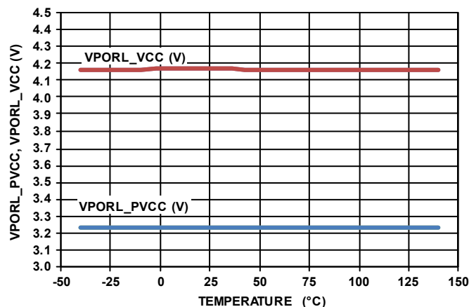
FIGURE 51. PVCC/VCC POR FALLING THRESHOLD vs TEMPERATURE
