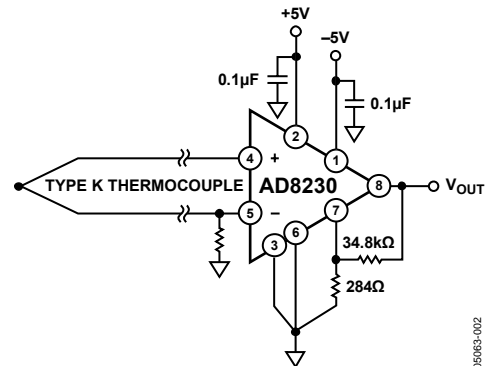
Figure 3. Thermocouple Measurement
