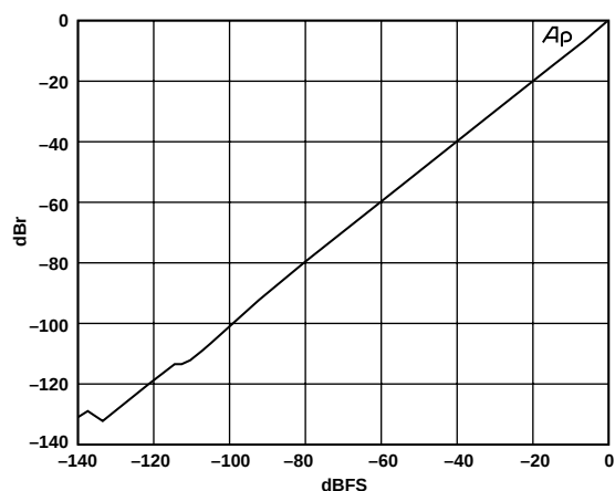
Figure 21. Linearity vs. Amplitude Input 200 Hz, SR 48 kS/s, 24-Bit Word
