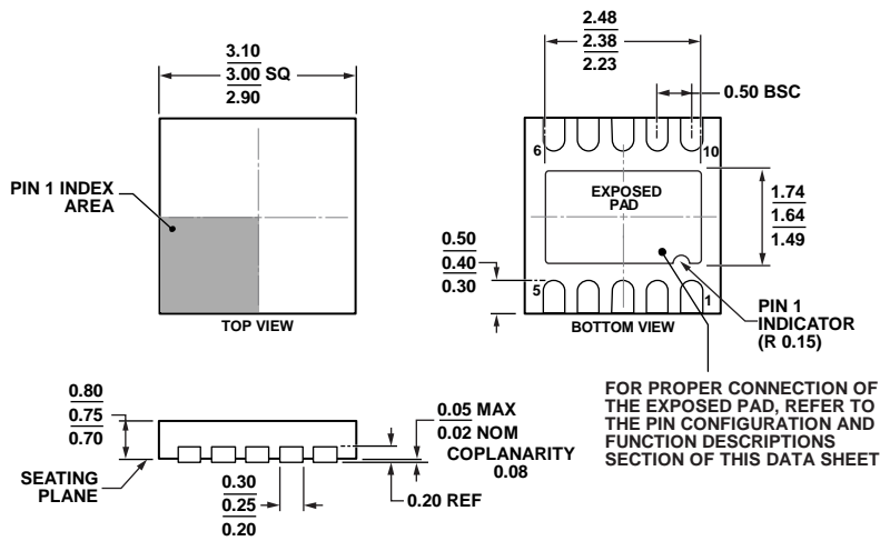
Figure 96. 10-Lead Lead Frame Chip Scale Package [LFCSF_WD] 3 mm × 3 mm Body, Very Thin, Dual Lead (CP-10-9) Dimensions shown in millimeters
