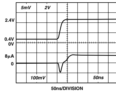
Figure 5. LSB Switching
