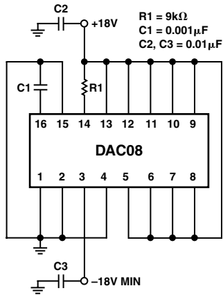
Figure 2. Burn-in Circuit
