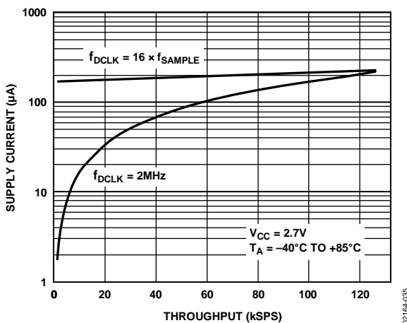
Figure 35. Supply Current vs. Throughput (μA)
