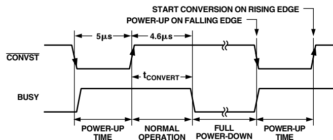
Figure 21. Using the \overline{\text{CONVST}} Pin to Power Up the AD7854 for a Conversion
