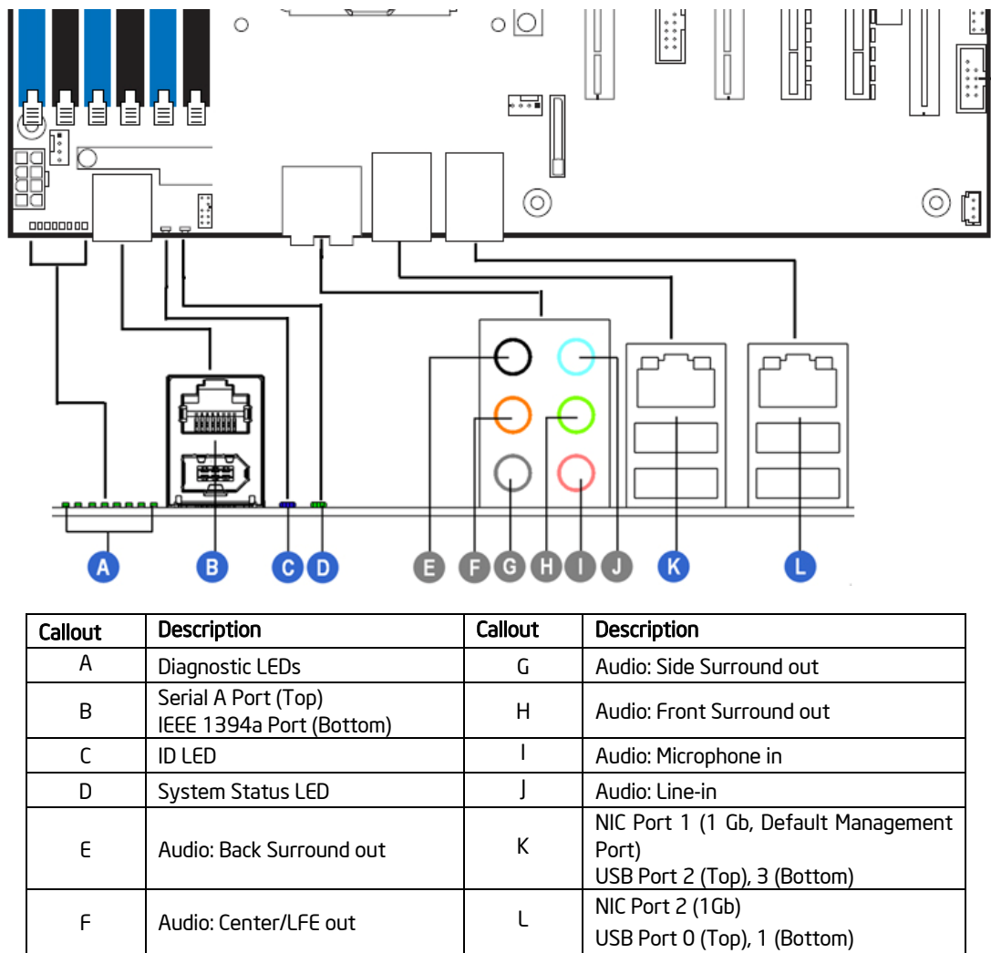
Figure 12. Intel® Workstation Board S5520SC Rear I/O Layout
