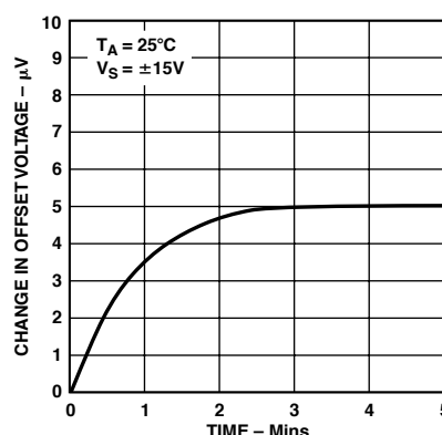
TPC 6. Warm-Up Offset Voltage Drift
