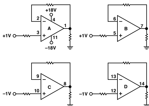
Figure 3. Burn-In Circuit
