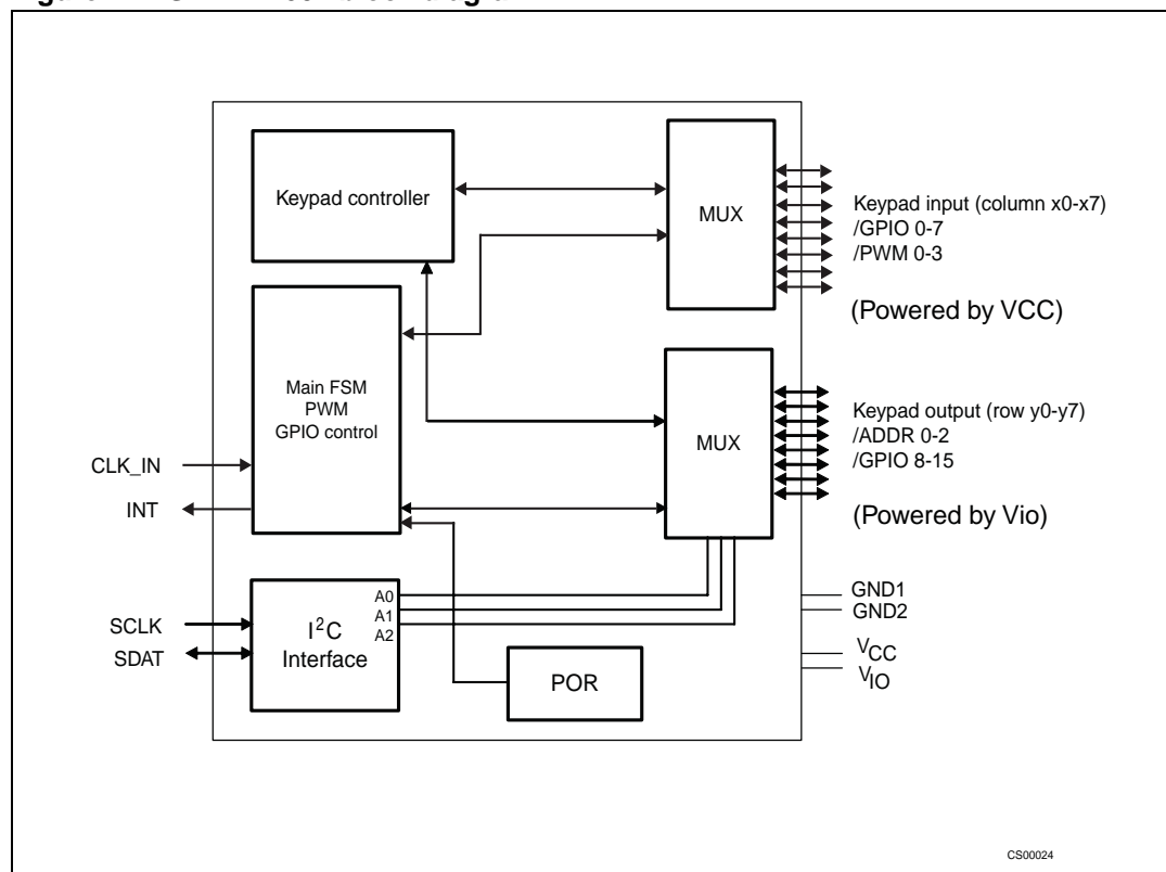
Figure 1. STMPE1601 block diagram
