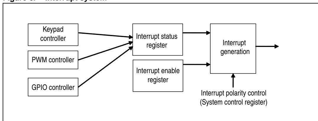
Figure 6. Interrupt system
