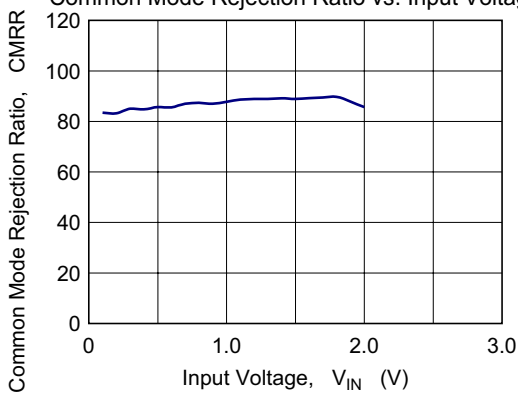
Figure 4-9 HA1631D04 Common Mode Rejection Ratio vs. Input Voltage
