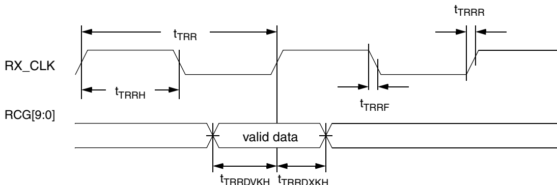
Figure 18. TBI Single-Clock Mode Receive AC Timing Diagram
