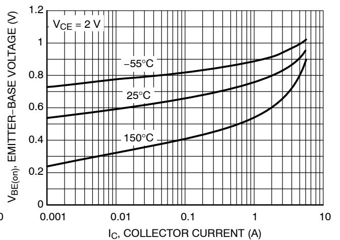
Figure 7. V_{BE(on)} Voltage
