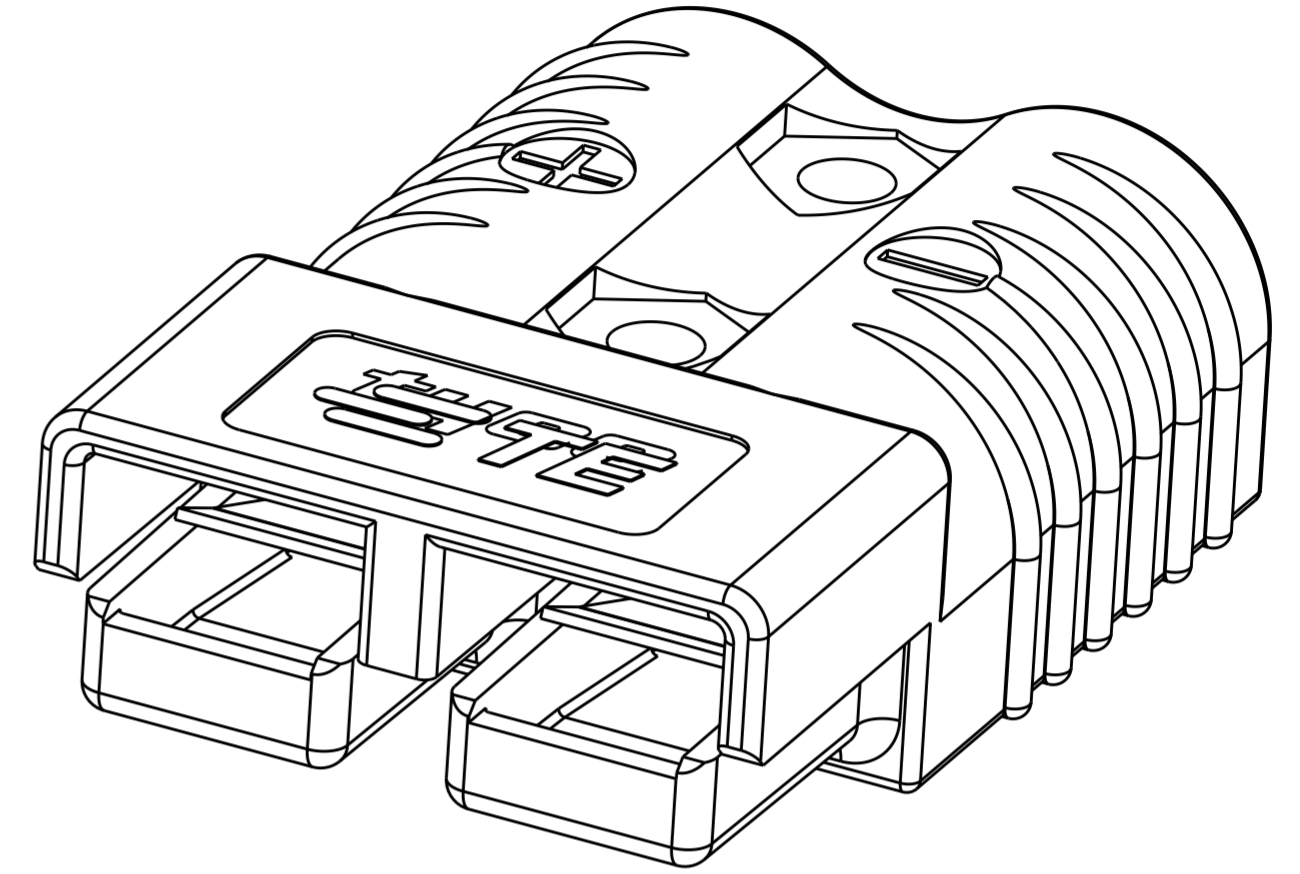
PART NUMBER: 1604043-4 WITHOUT CONTACT SHOWN
