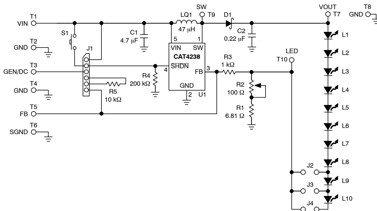
Figure 1. CAT4238AEVB Board Schematic
