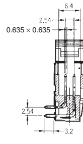
Right-angle DIP terminals
