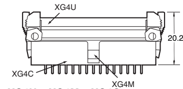
XG4U + XG4M + XG4C (With right-angle terminals)
