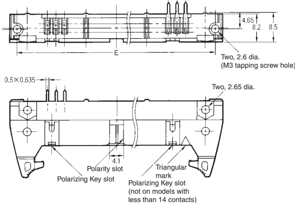
Mounting holes (bottom view) Right-angle terminals
