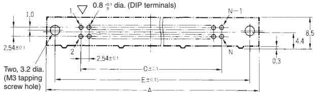
Straight terminals
