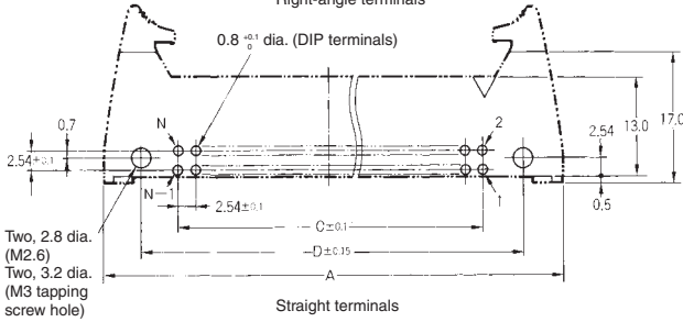
Straight terminals
