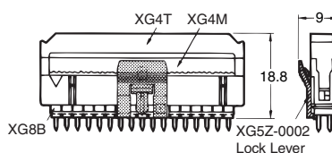
XG4T + XG4M + XG8B (Original Plug) + Lock Lever
