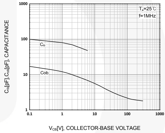
Figure 4. Capacitance
