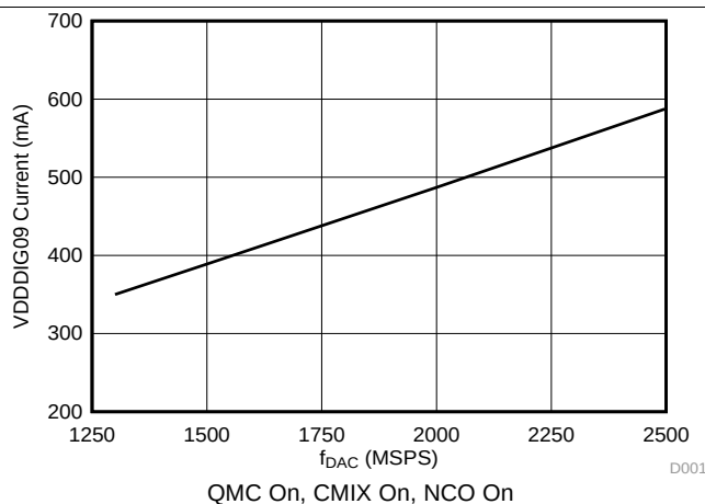
Figure 33. VDDDIG09 Current vs f_{\text{DAC}}
