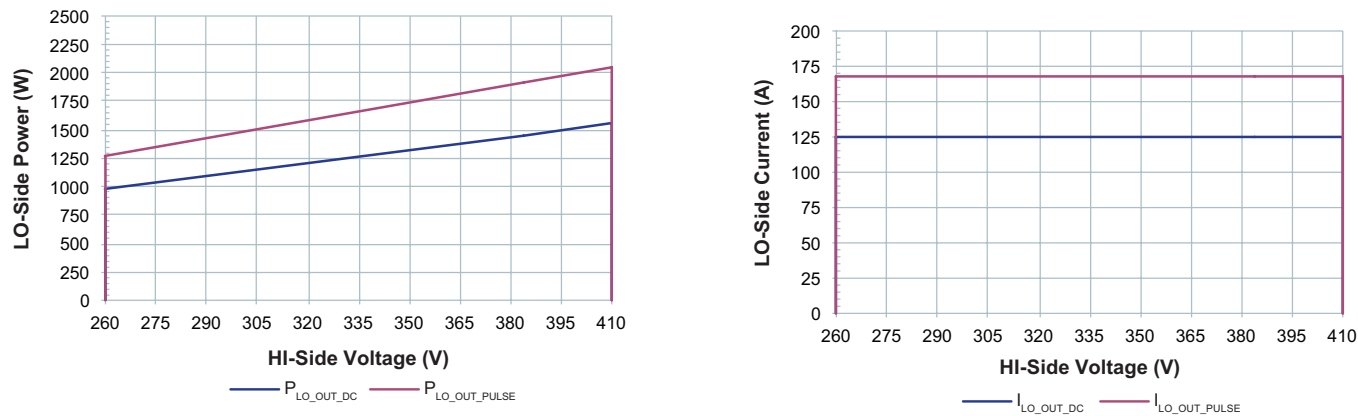
Figure 2 — Specified electrical operating area using rated R_{LO\_HOT}
