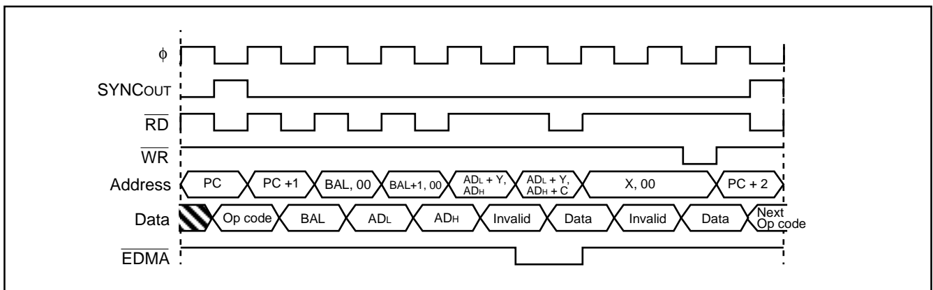
Fig. 78 LDA ($zz), Y instruction sequence when \overline{EDMA} enabled and T flag = "1"
