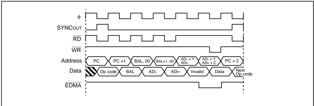
Fig. 76 STA ($zz), Y instruction sequence when \overline{EDMA} enabled
