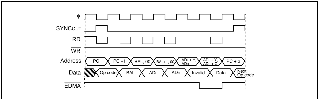
Fig. 77 LDA ($zz), Y instruction sequence when \overline{EDMA} enabled and T flag = "0"
