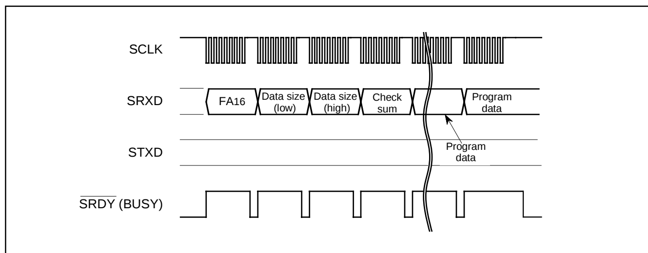
Fig. 111 Timing for download
