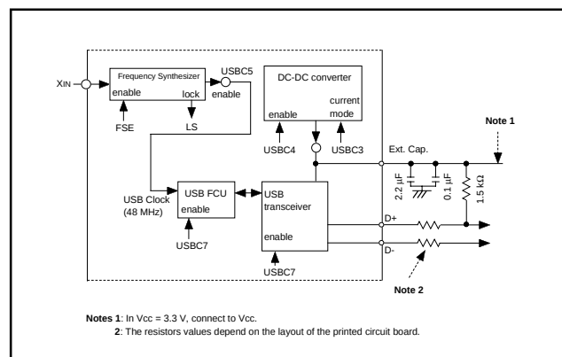
Fig.125 Peripheral circuit
