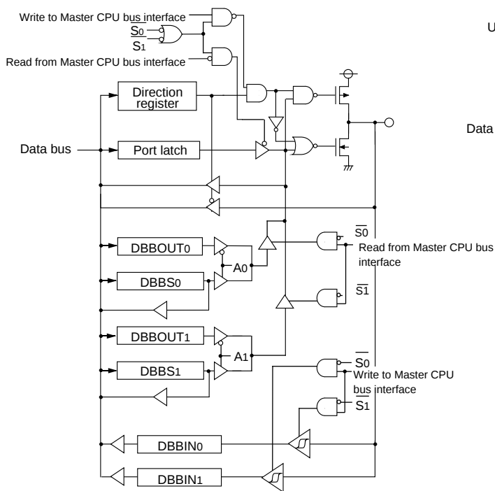
(11) Port P6
