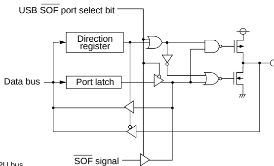
(12) Port P70
