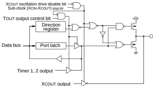
(9) Port P53
