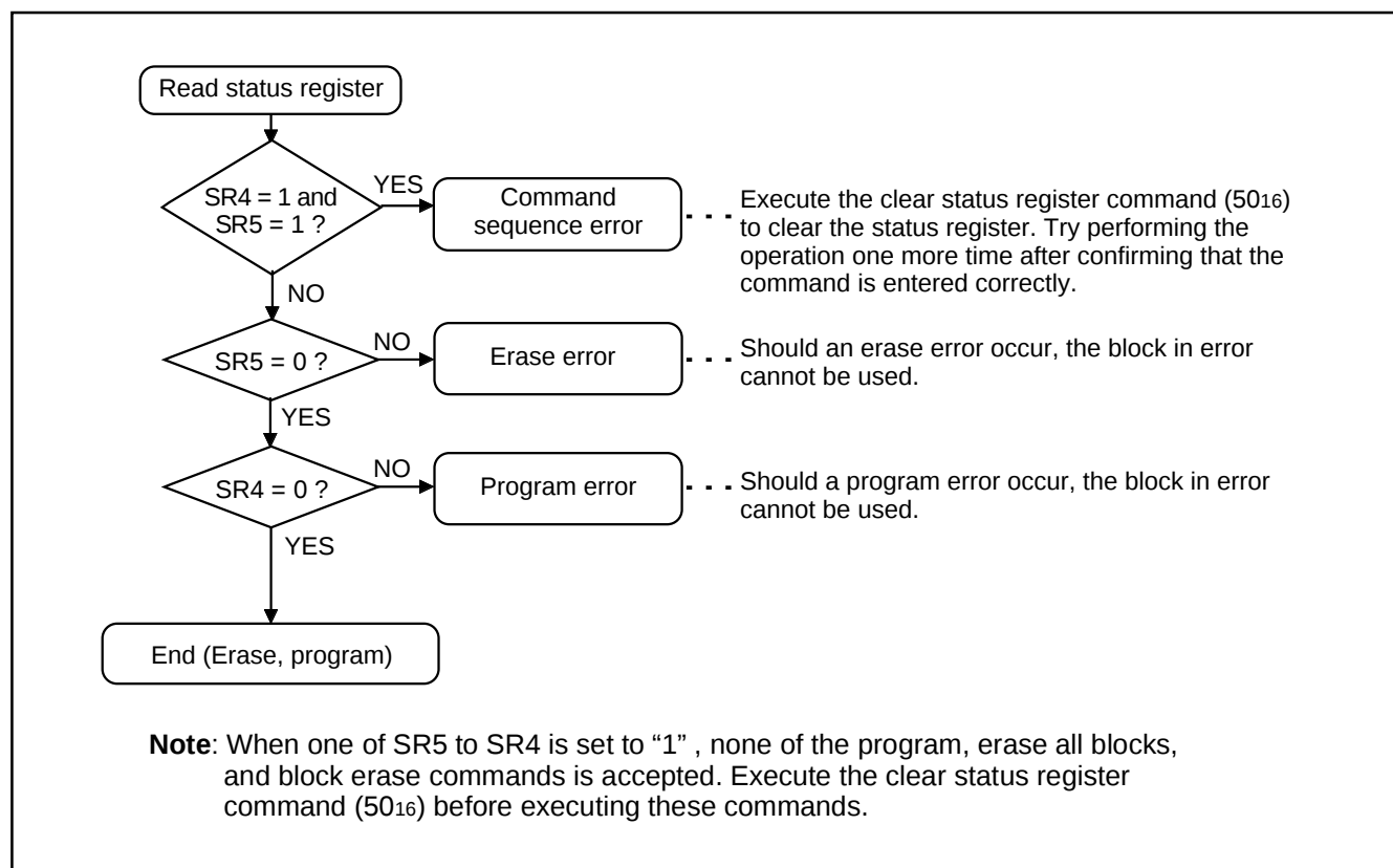
Fig. 116 Full status check flowchart and remedial procedure for errors
