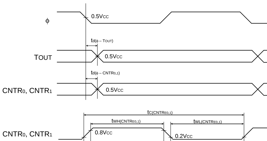
Fig. 81 Timing diagram (1)
