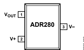
Figure 2. 3-Lead SC70 (KS Suffix)
