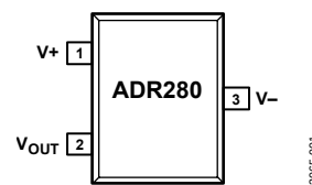
Figure 1. 3-Lead SOT-23 (RT Suffix)
