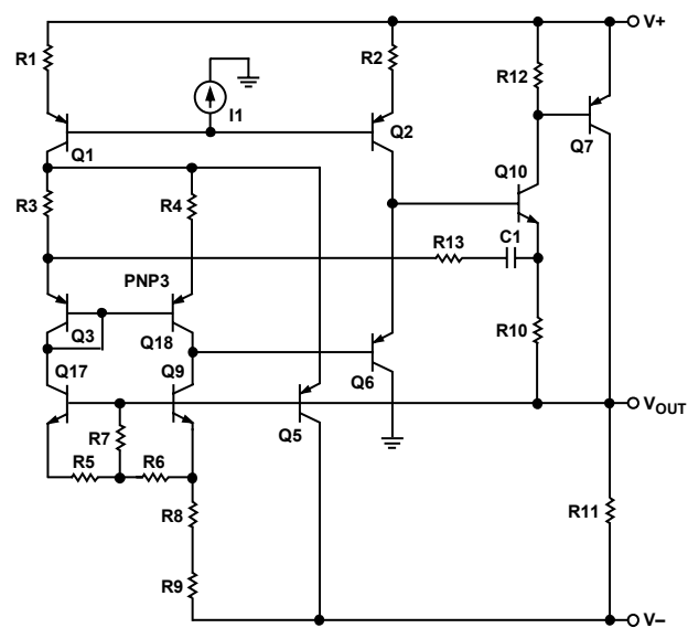
Figure 11. Simplified Architecture
