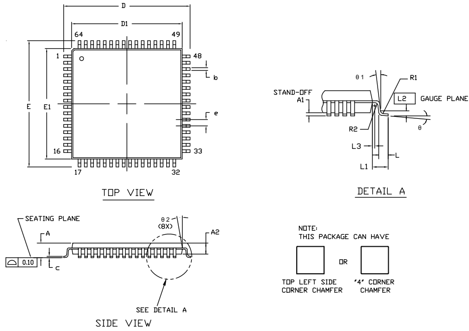
Figure 7. 64-Pin 14 × 14 × 1.4 mm TQFP Package Outline
