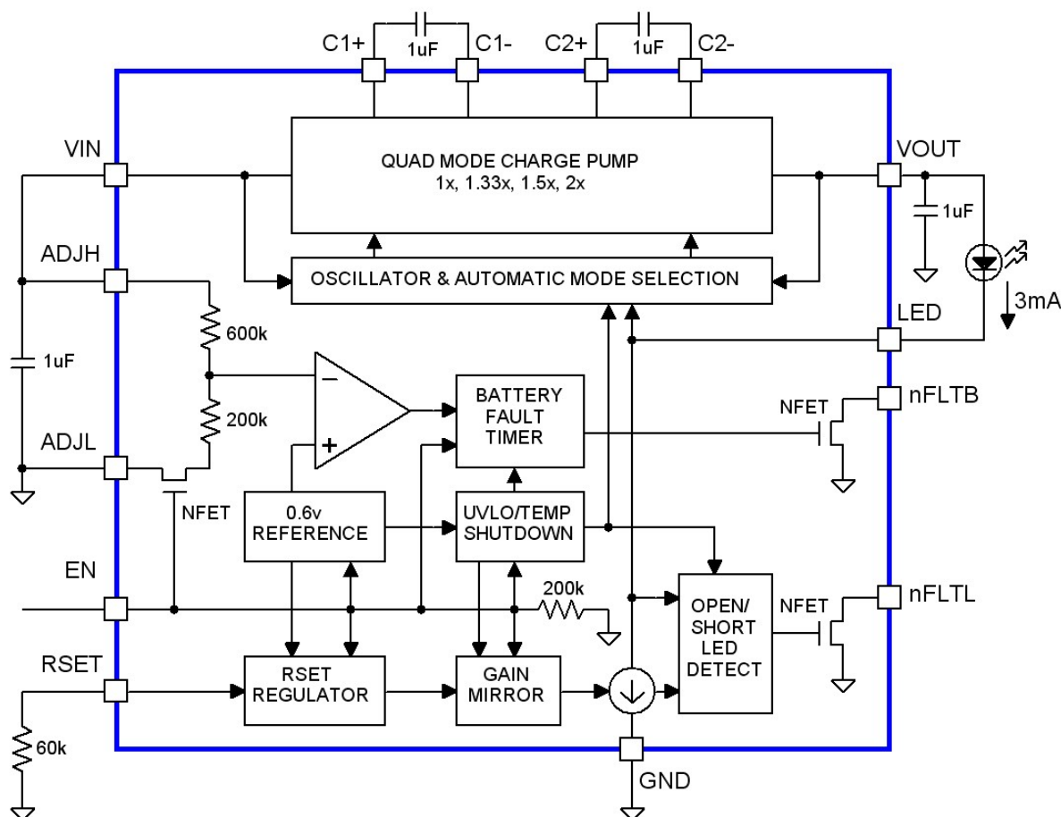
Figure 24. CAT3661 Functional Block Diagram
