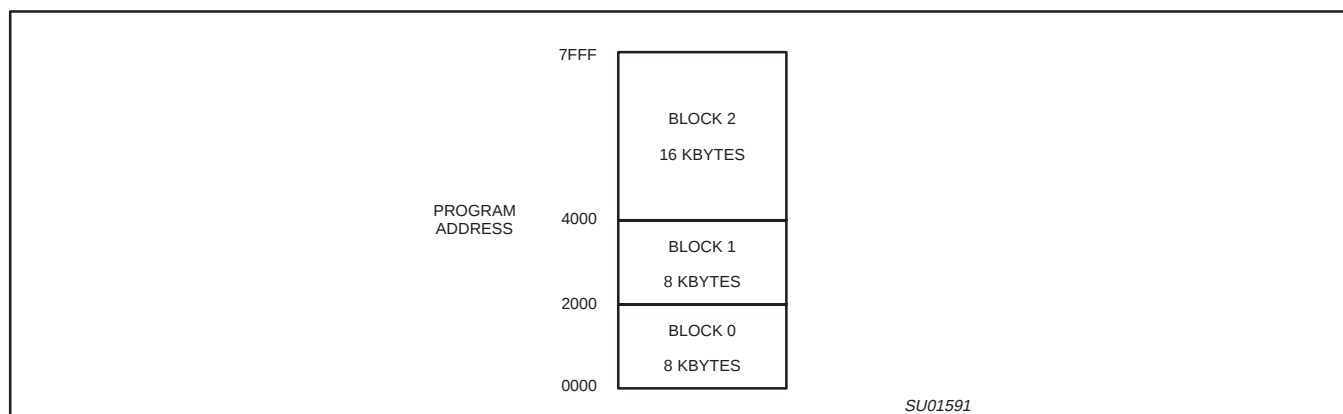
Figure 3. Flash Memory Configuration
