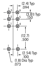
Double Pole
