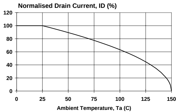
Fig.2. Normalised continuous drain current. ID\% = 100 \cdot I_D / I_{D\ 25\ ^\circ C} = f(T_a) ; conditions: V_{GS} \leq -10\ V
