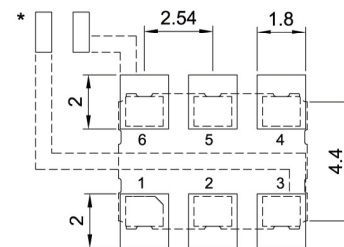
Top View Suggested Layout
